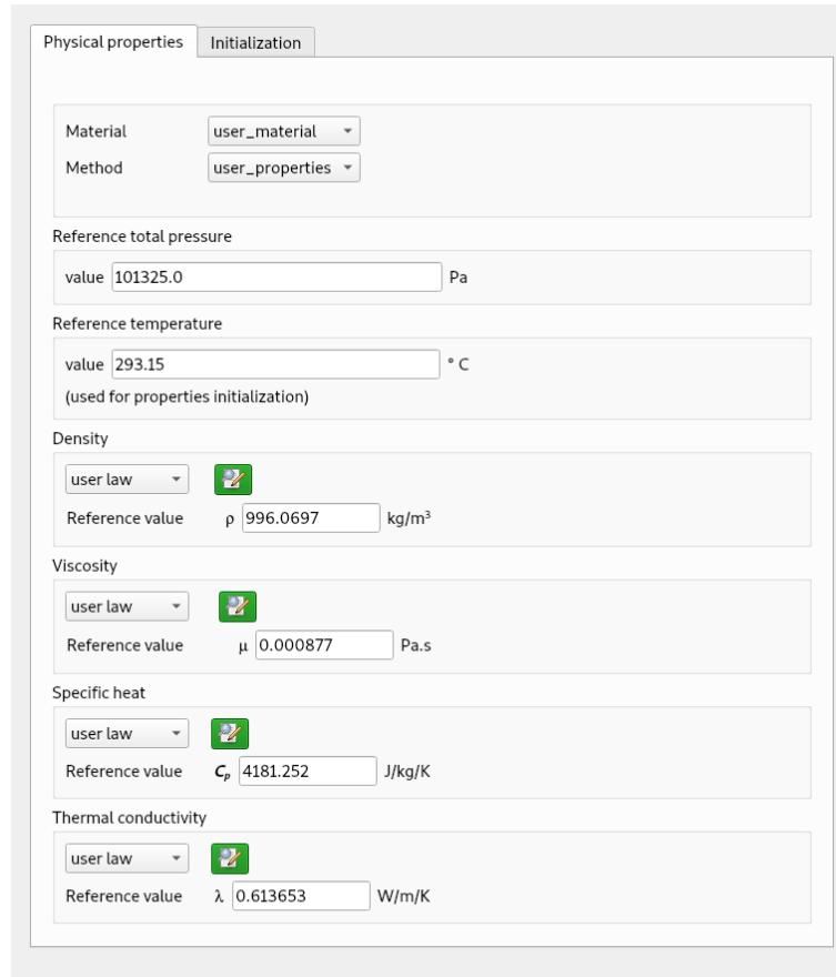
Figure III.6: Selection of fluid properties.
