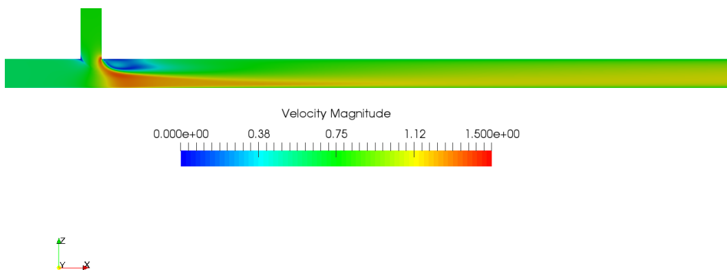
Figure III.29: Velocity magnitude field in the plane (xz).
