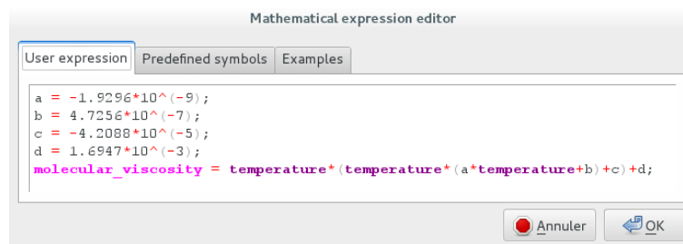
Figure III.10: Coding the viscosity as a function of the temperature.
