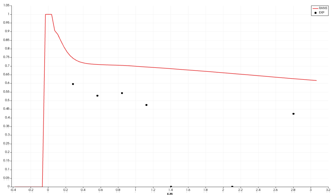
Figure IV.3: Dimensionless temperature along the lines defined in the main pipe at y=0 and z=0.07 .
