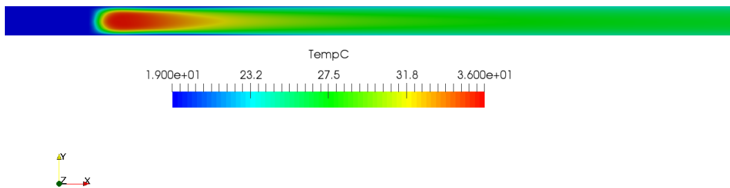
Figure III.28: Temperature field in the plane (xy).
