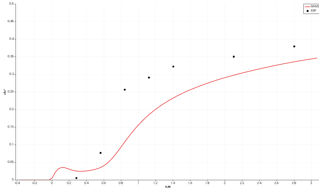
Figure IV.4: Dimensionless temperature along the lines defined in the main pipe at y=-0.07 and z=0 .
