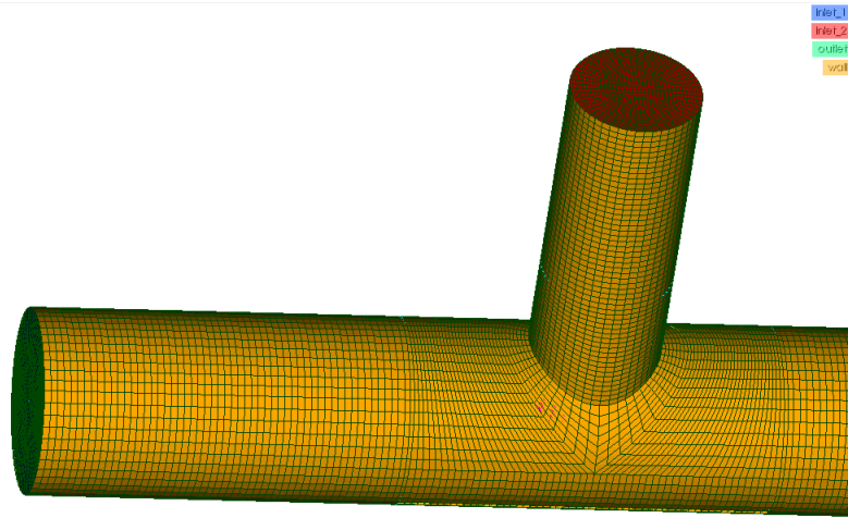
Figure VII.22: Zoom on final mesh
