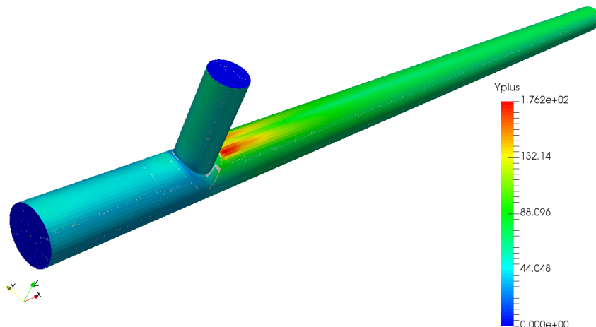
Figure III.26: Visualisation of the y^+ on ‘CellDataPointData2’.
