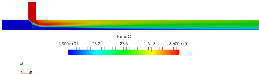
Figure III.27: Temperature field in the plane (xz).
